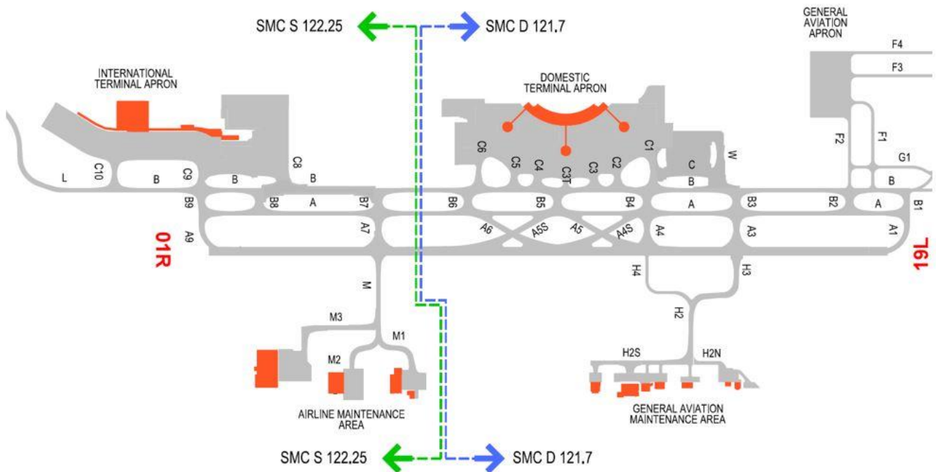
Figure 50 – SMC S & SMC D Radio Frequency Split map
